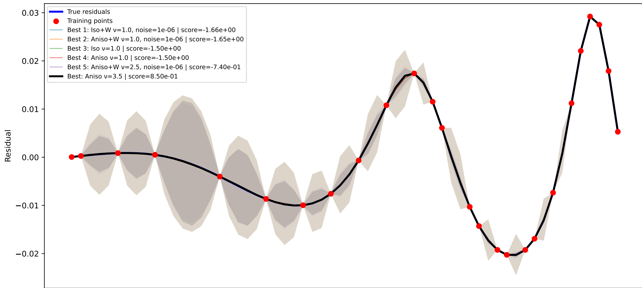
GPR kernel comparison node=24 RMSE=1.961e-05, train RMSE=1.328e-11
